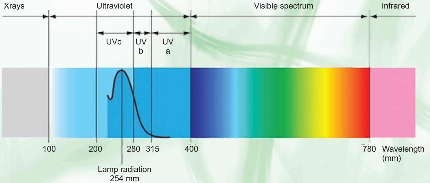
Fig: Spectrum of radiations
