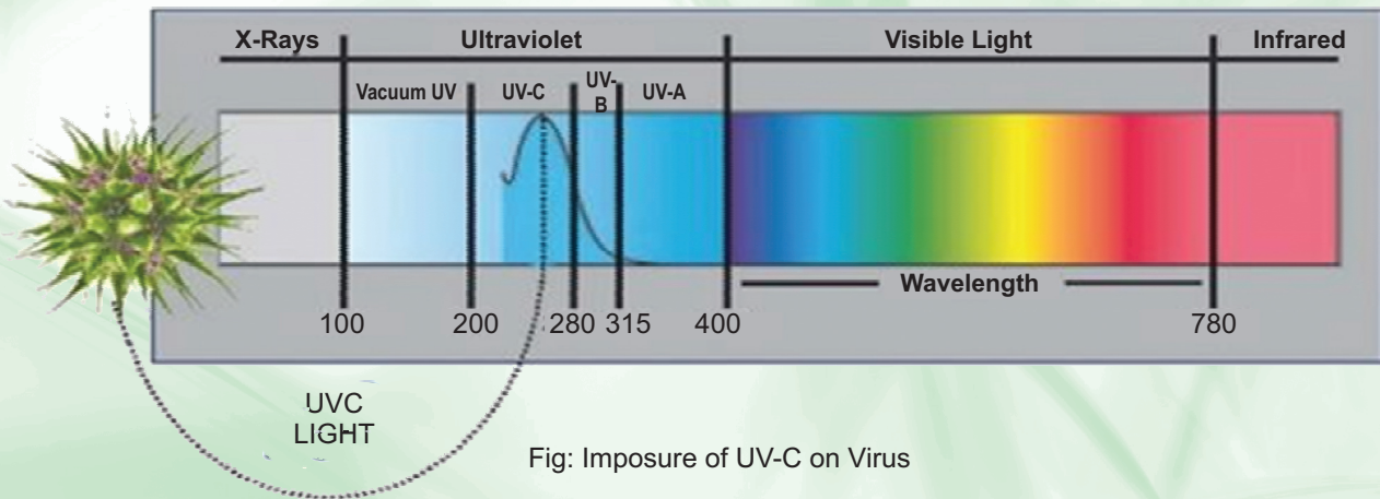
Fig: Spectrum of radiations
