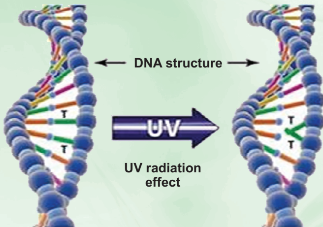
Fig: Effect of UV-C on DNA
